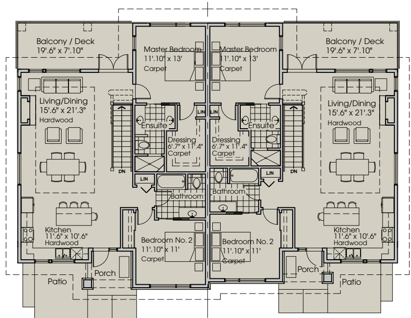
MAIN FLOOR PLAN - DUPLEX UPHILL
