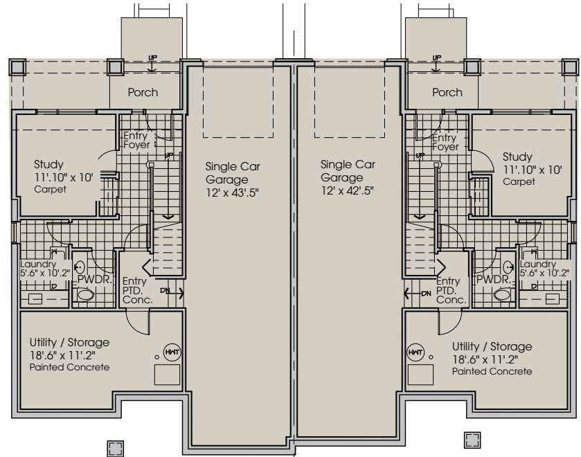
LOWER FLOOR PLAN - DUPLEX UPHILL
